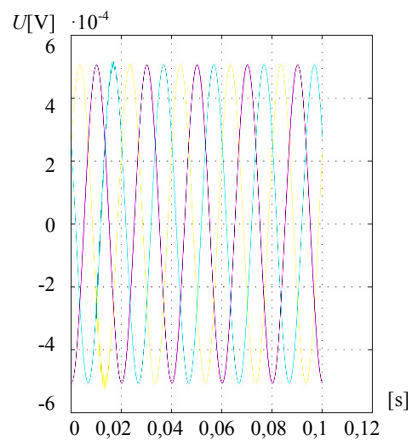
Fig. 3. Phase to phase voltage of all three phases before and after fault, isolated neutral point, case A.
